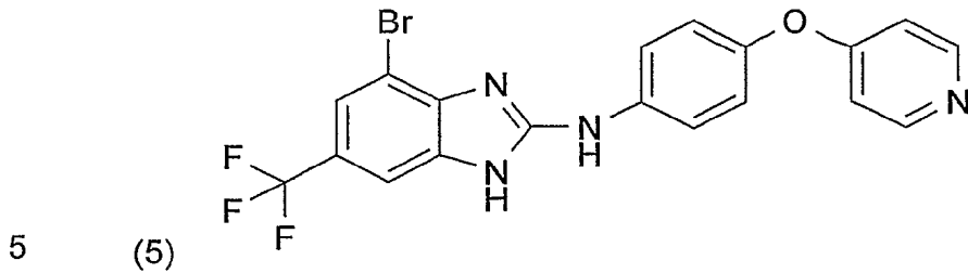
(4-Brom-6-trifluormethyl-1H-benzimidazol-2-yl)-[4-(pyridin-4-yloxy)-phenyl]-amin
